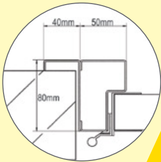
Frame dimensions
